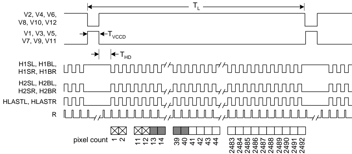
Figure 11: Line Timing Dual Output
