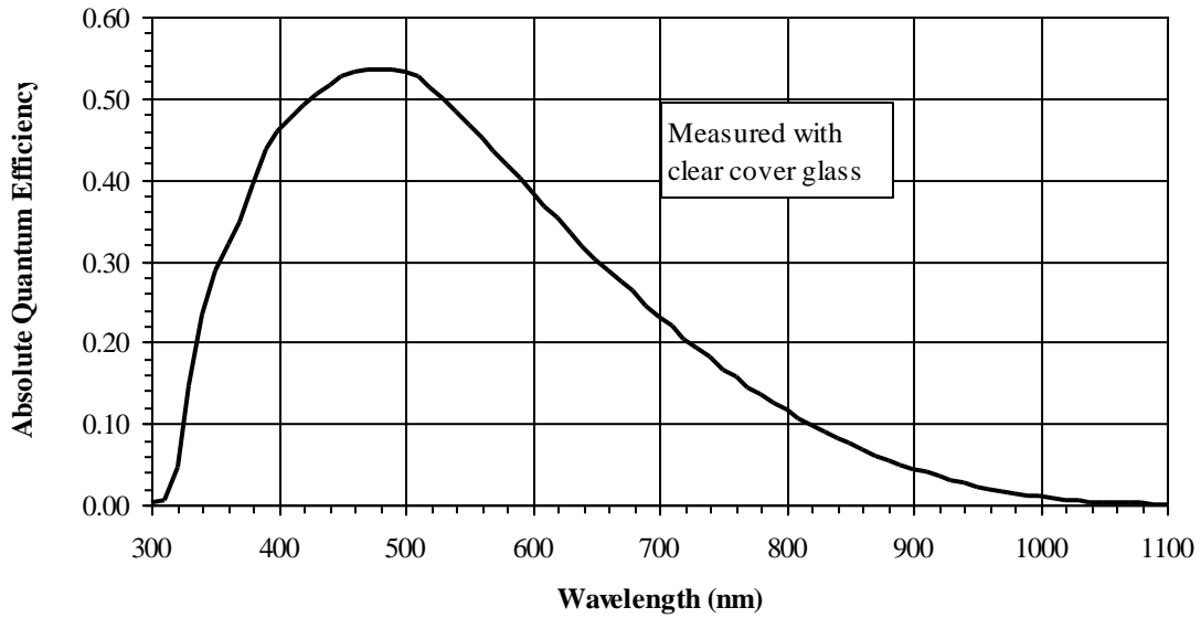
Figure 5: Monochrome with Microlens Quantum Efficiency
