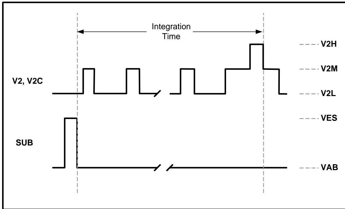
Figure 18: Integration Time Definition
